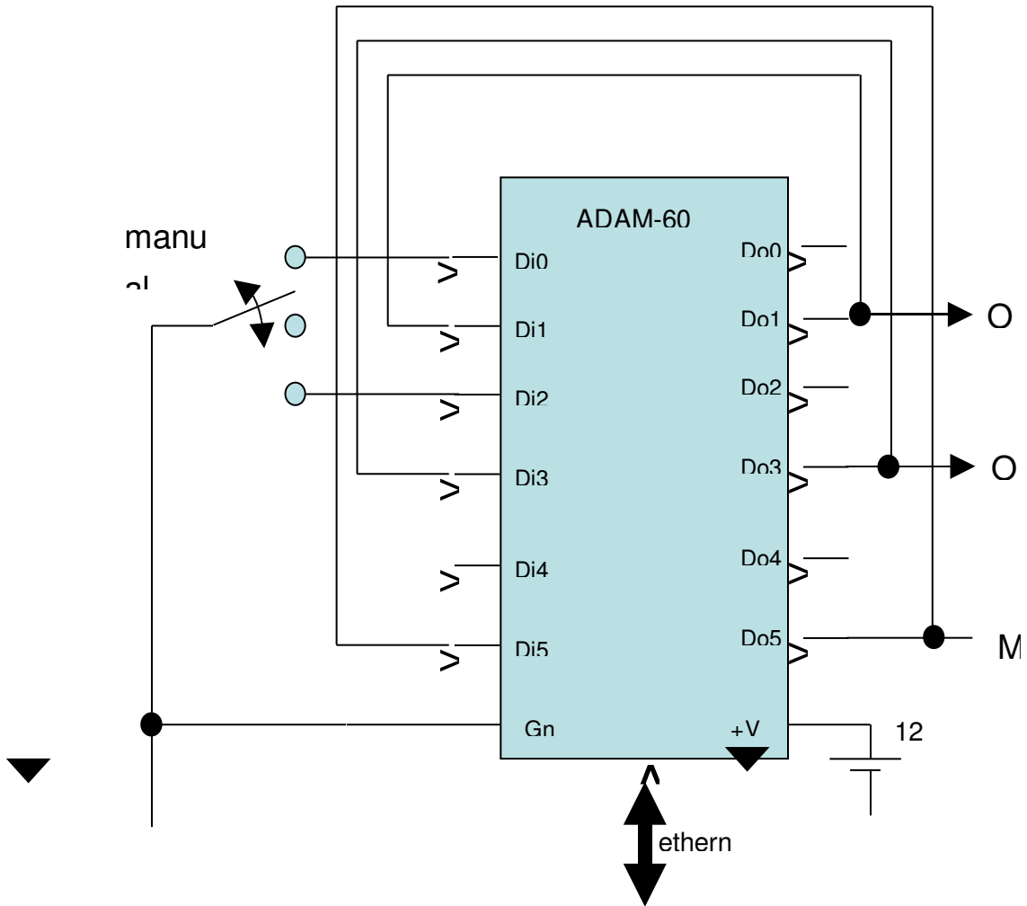
Figure 1: External wiring of the ADAM module
