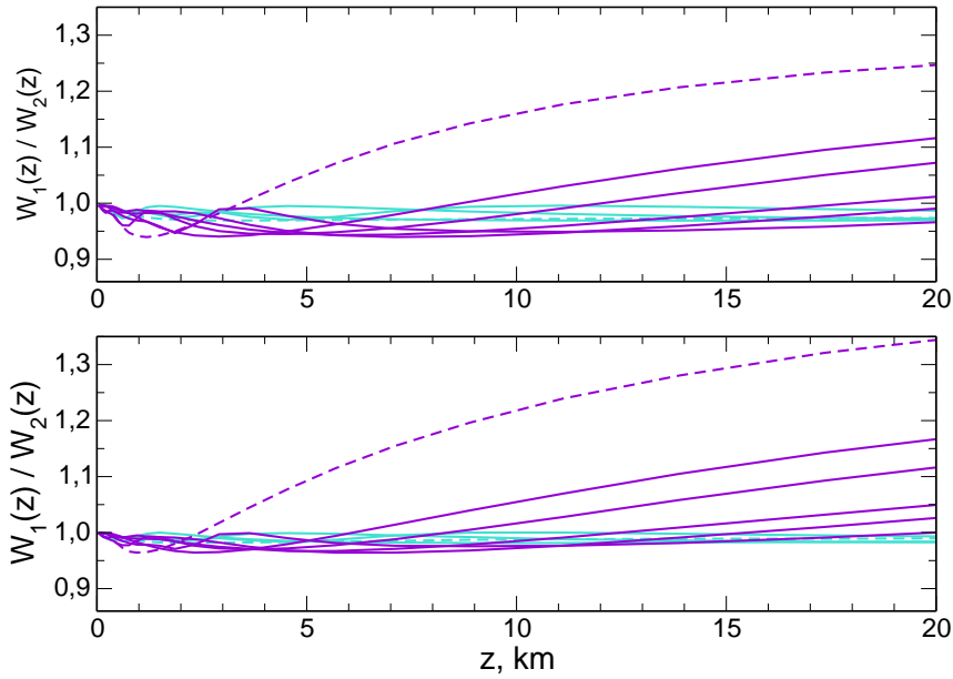
Figure 4: Upper plot: the ratio of WF(without) to WF(without_cut). Lower plot: the ratio of WF(elt.mass_dimm) to WF(mass). These bands differ in \Delta\lambda and are similar in \lambda_0 .
