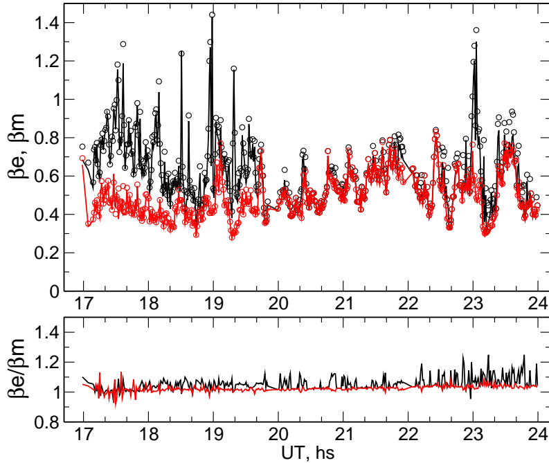
Figure 5: Upper plot: Data of the original MASS device at Maidanak for 2005-08-26. The seeing values \beta_E and \beta_M are computed from the profiles restored with the elt_mass_dimm (circles) and with the mass (line) curves, respectively. Lower plot: the ratio \beta_E to \beta_M (black — including the 0.5 km layer, red — without this layer).
