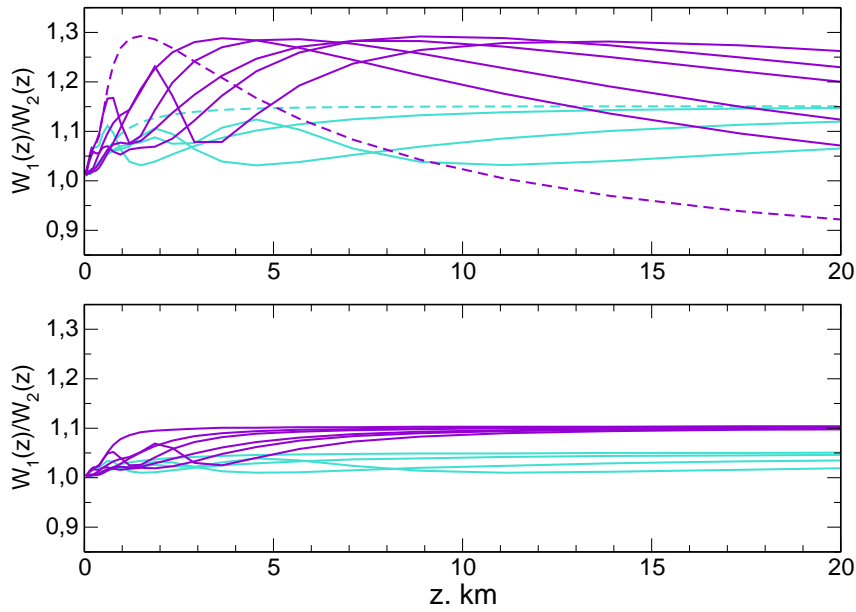
Figure 3: Upper plot: the ratio of WF(eso_md) to WF(mass_dimm). Lower plot: the ratio of WF(eso_md) to WF(shifted by 20 nm eso_md). The green curves are the normal indices, the violet curves are the differential ones. The dashed curves correspond to the A and AB indices.
