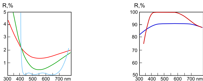
Figure 1: Reflectance of a refractive surface with AR coating (on the left). Red curve — \text{MgF}_2 film on BK7 glass, green — \text{MgF}_2 on SF5 glass, blue curve — enhanced multilayer coating for visual light. On the right — reflectance of Al layer without AR (blue) and with visual AR coating (red).
