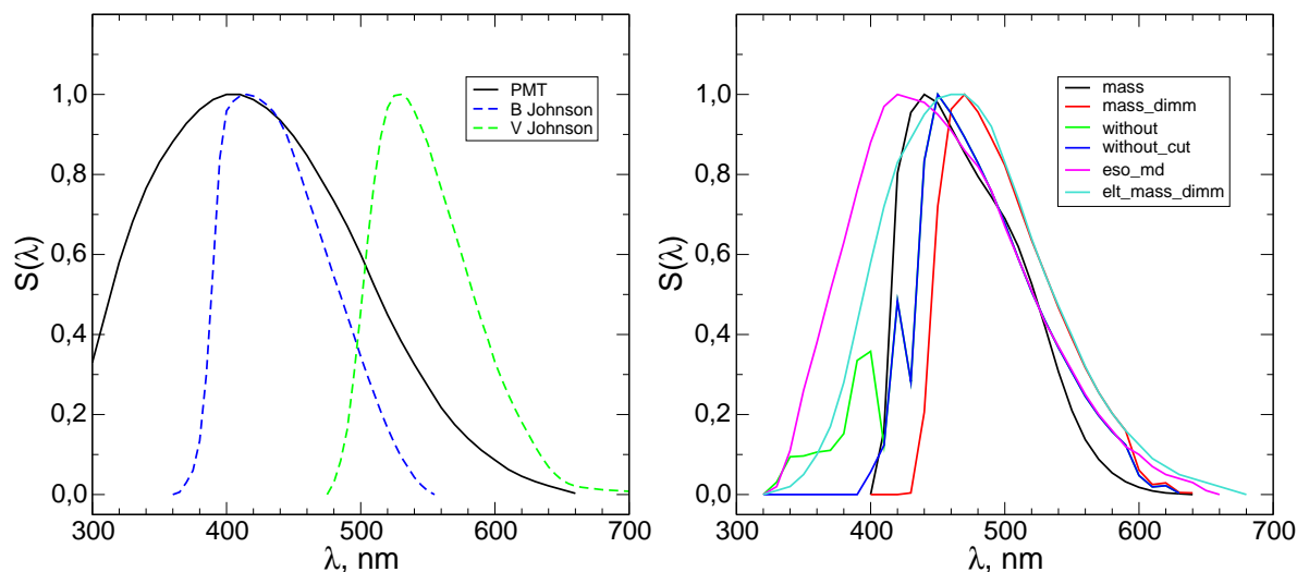
Figure 2: On the left: Photon spectral sensitivity of the PMT R7400 from Hamamatsu and the standard photometric bands B and V . On the right: The collection of the MASS spectral response curves.
