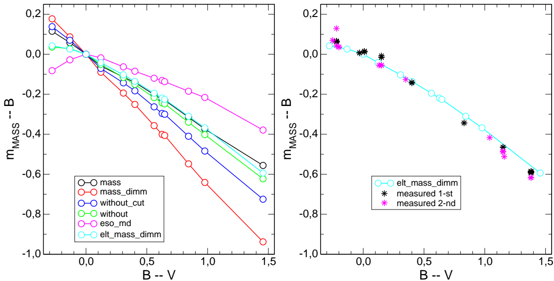
Figure 6: On the left: The calculated color-color diagram m_{MASS} - B vs. B - V for all MASS spectral response curves. On the right: The color equation for the elt_mass_dimm (line) and the measurements made with the ESO MASS/DIMM (points).
