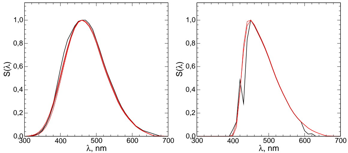
Figure 8: On left: the original curve elt_mass_dimm used to compute the simulated colors m_{MASS} - B (black) and a few response curves restored from these colors with different noise realizations (red). On right: the same for without_cut .
