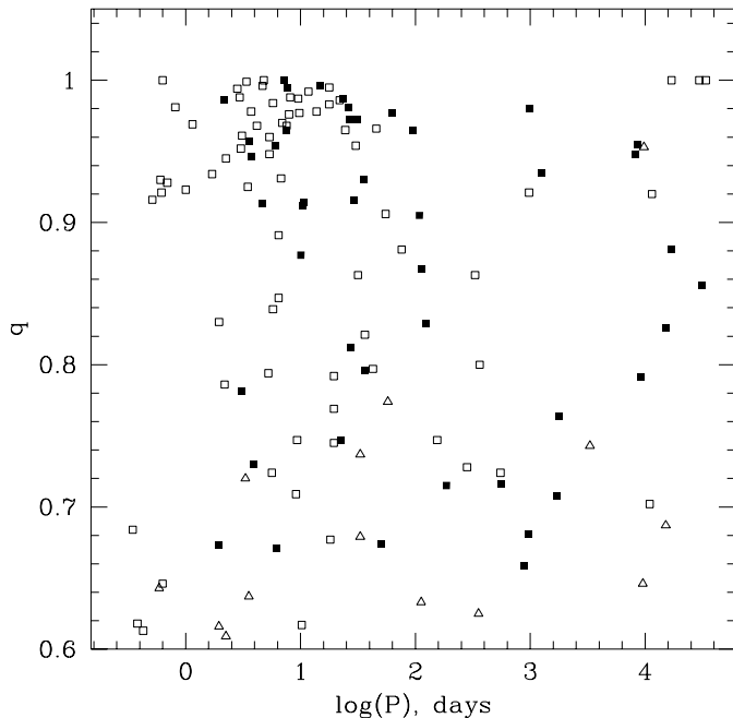
Fig. 1. Mass ratio of solar-type double-lined spectroscopic binaries is plotted against the logarithm of their orbital period in days. Empty squares - data from the Batten et al. (1989) catalogue, filled squares - recent orbits (SB+). Triangles show the lower mass ratio limits for single-lined binaries from Batten et al. (1989).
