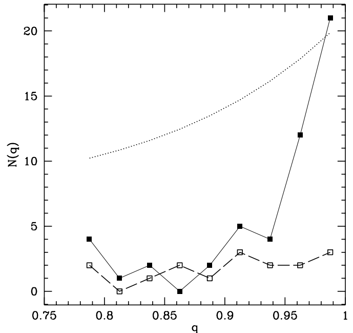
Fig. 2. The mass ratio distribution in the two period ranges: short, 2–30 days (full line and filled symbols, 52 systems) and long, 50–10000 days (dashed line and empty symbols, 15 systems). The number of objects in 0.025 bins in q is plotted on the vertical axis. Dotted line indicates possible sample bias as discussed in the text.
