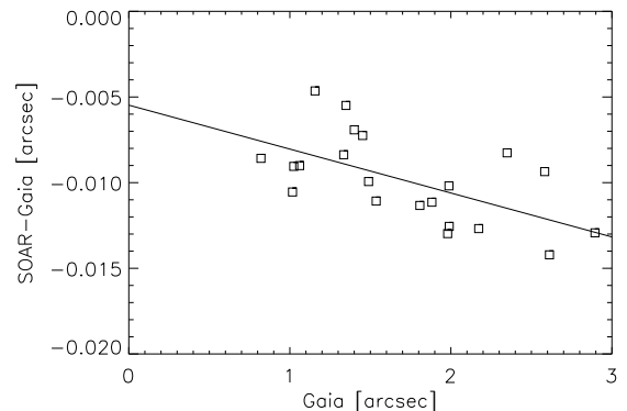
FIG. 3.— Comparison between SOAR and Gaia separations of calibration binaries. The line is a linear fit given by Equation 1.
