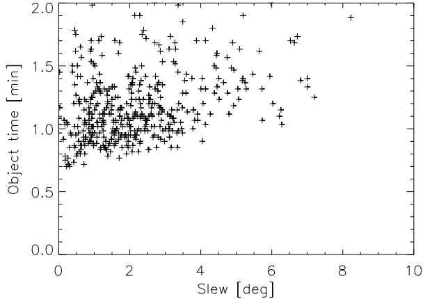
FIG. 1.— Correlation between observing time per object and the slew distance for the night of 2018 April 3/4. The vertical axis plots time between observations of successive objects.
