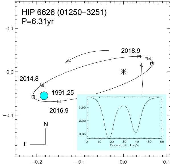
FIG. 7.— Orbit of HIP 6626 (HDS 184, WDS J01250-3251). The primary component is located at the coordinate origin, with scale in arcseconds. The ellipse marks the trajectory. The original Hipparcos discovery is marked by the blue circle, the SOAR measures from 2014.8 to 2018.9 by squares. The insert shows double lines observed on 2018.916, shortly after the periastron passage.
