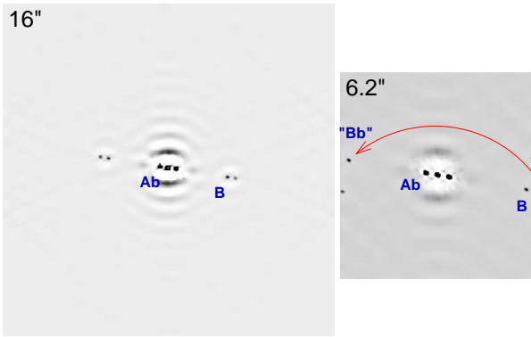
FIG. 9.— Triple system 07185–5724. The left panel shows ACF of the data cube recorded in 2018.2 with the full field; the peaks corresponding to the companions Ab at 0''.4 and B at 2''.9 are indicated. In the right panel, the ACF in the 6''.2 field is shown. The peak corresponding to the correlation between Ab and B (red circle) falls outside the field and is aliased (reflected) to a different position (red arrow), creating an illusion of another companion Bb.
