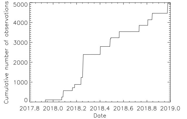
FIG. 2.— Cumulative plot of the number of HRcam observations at SOAR during 2018 (all programs).
