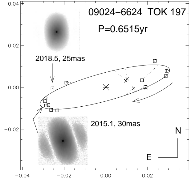
FIG. 8.— Orbit of \alpha Vol (WDS J09024-6624). The inserts show power spectra recorded in 2015.1 near maximum separation and in 2018.5 at separation of 25 mas. Crosses denote non-resolutions.
