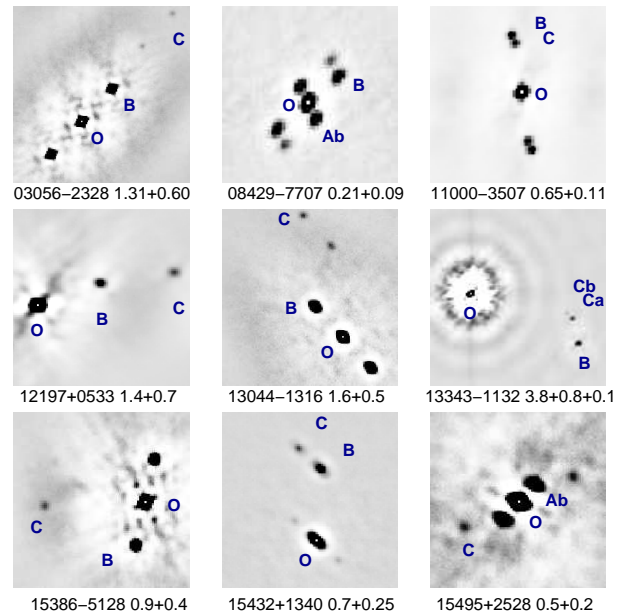
FIG. 6.— Fragments of ACFs of new triple systems with comparable separations between components (trapezia). North up, East left, scale arbitrary. The WDS code and separations in arcseconds are given below each fragment; the peaks corresponding to the locations of the components are indicated by letters; other peaks are their symmetric counterparts and cross-correlations between the two secondaries (an ACF of a triple star contains 6 peaks). The central peak of the ACF is marked by the white dot and the letter O.
