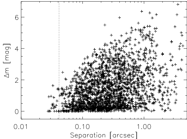
FIG. 4.— Magnitude difference in the I band vs. separation for pairs resolved in this filter. The vertical dotted line marks the formal diffraction limit of 41 mas.
