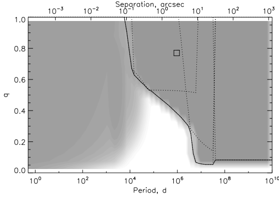
FIG. 8.— Probability of companion detection for HIP 55 ( p_{\text{HIP}} = 15.4 mas). Individual limits for resolved companions from Hipparcos , WDS, 2MASS, and CPM are plotted in dotted lines, the combined limit – in full line. No data from AO or speckle interferometry are available for this target. The visual companion B at 3.8'' (square) is listed in the WDS and 2MASS. The gray shading shows the combination of spatial resolution with limits resulting from Hipparcos acceleration \Delta\mu and from the five RV measurements over time interval T = 1394 d by Nordström et al. (2004).
