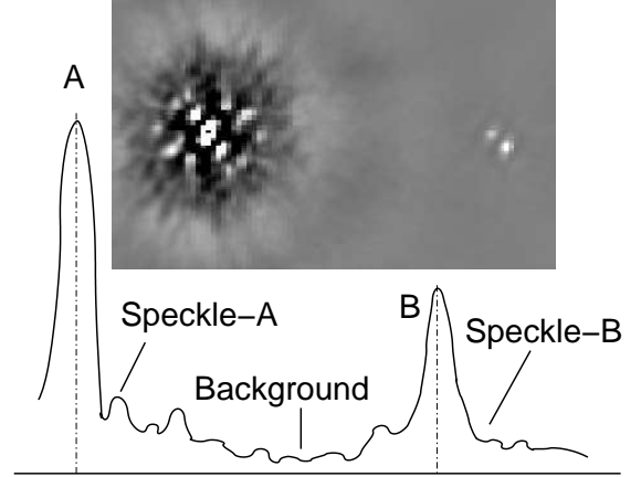
FIG. 6.— Detection of sub-systems in the secondary components of resolved binaries. The image shows detection of the sub-system Ba,Bb ( 0''.12 , \Delta m = 0.9 ) in the binary HIP 44874 AB ( 1''.79 , \Delta m = 4.8 ) observed with speckle interferometry at SOAR in 2013. The curve illustrates noise in the image of a binary, dominated by the residual speckle structure near each component and by the background fluctuations away from them.
