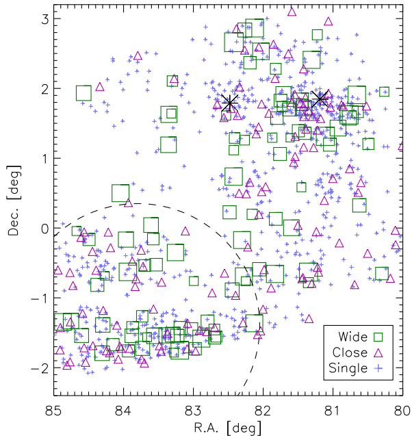
FIG. 20.— Spatial distribution of single stars (blue crosses), close Gaia binaries (magenta triangles), and wider VISTA Orion binaries (green squares). The size of the squares reflects binary separation ranging from 0''.6 to 10'' . The two black asterisks show the locations of 25 Ori and HR 1833. The dashed circle depicts the boundary of Ori OB1b.
