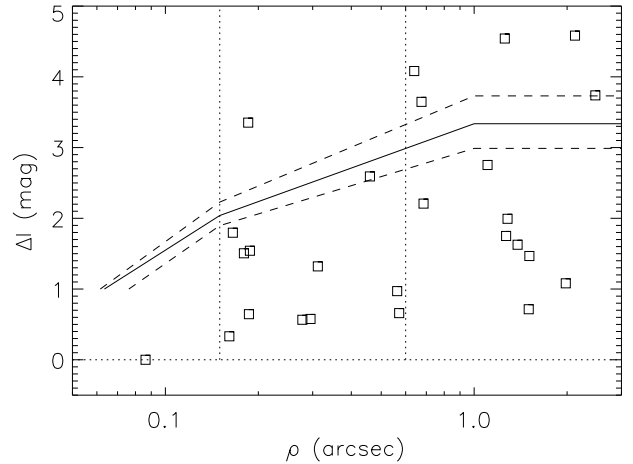
FIG. 15.— Separations \rho and magnitude differences \Delta I of CVSO pairs resolved at SOAR (note: 2 pairs with respective separation of 3''.7 and 3''.1 are outside the plotting area). The full and dashed lines show the median detection limit and its quartiles. The separation range between 0''.15 and 0''.6 used in the statistical analysis is delimited by the vertical dotted lines.
