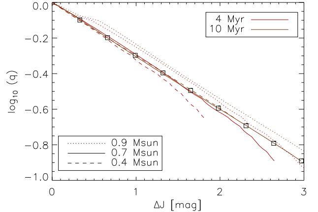
FIG. 16.— Relation between \log_{10} q and \Delta J derived from the PARSEC isochrones for primary stars of 0.4, 0.7, and 0.9 M_{\odot} mass and companions more massive than 0.075 M_{\odot} . Squares correspond to the linear formula \log_{10} q = -0.3\Delta J .
