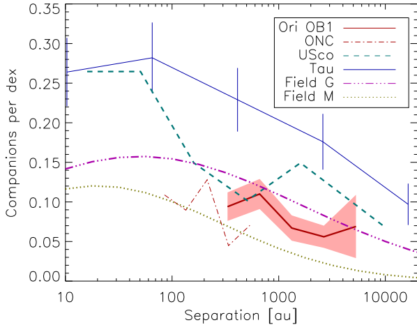
FIG. 22.— Comparison of multiplicity in different populations (see text).
