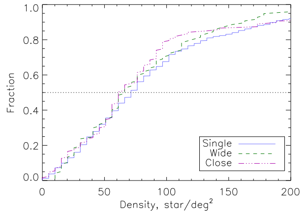
FIG. 21.— Cumulative distributions of the density of association members around single stars, wide, and close binaries, computed for 0''.25 radius.
