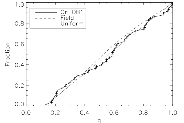
FIG. 17.— Cumulative distribution of the mass ratio q for 58 binaries with separations between 1''.2 and 5'' (line and crosses). The dashed and dotted lines correspond to the field binaries (see the text) and to the uniform distribution, respectively.
