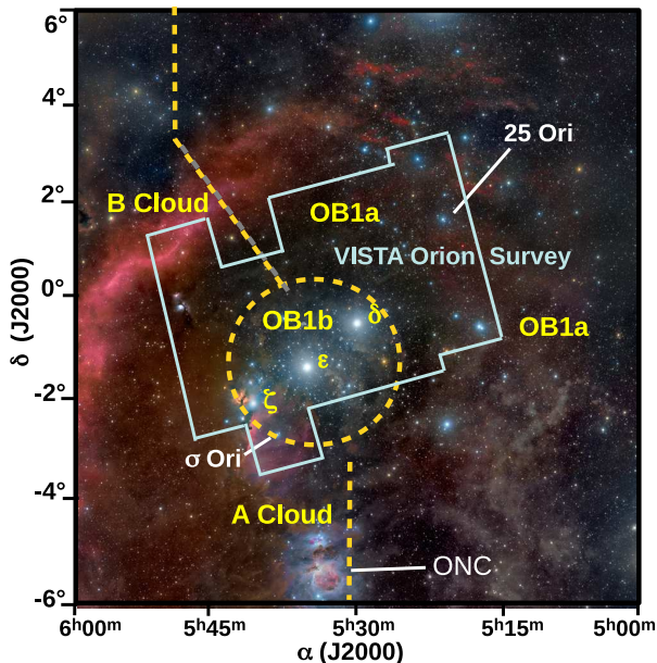
FIG. 1.— Wide field optical image of the area encompassed by the CVSO in the Orion OB1 association, showing as an irregular polygon the approximate footprint of the VISTA Orion Survey (Petr-Gotzens et al. 2011). The Orion OB1b sub-association is the region within the dashed line circle, as in Briceño et al. (2005). The OB1a sub-association is the area to the west of the OB1b region and the dashed lines north and south of it, which roughly mark the limits of the Orion A and B molecular clouds, as indicated by the labels. We also indicate the location of the three Orion belt stars \delta , \epsilon , and \zeta Ori, as well as the \sigma Ori and 25 Ori clusters. The Orion Nebula Cluster (ONC) is also indicated. Photo courtesy of Rogelio Bernal Andreo ( http://www.deepskycolors.com/ ).
