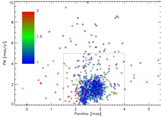
FIG. 4.— Correlation between parallax and total PM for our sample. The symbols are colored according to the excess error r_w , as shown by the color bar. The dotted box shows the limits of parallax and PM adopted for the 934 astrometric members.
