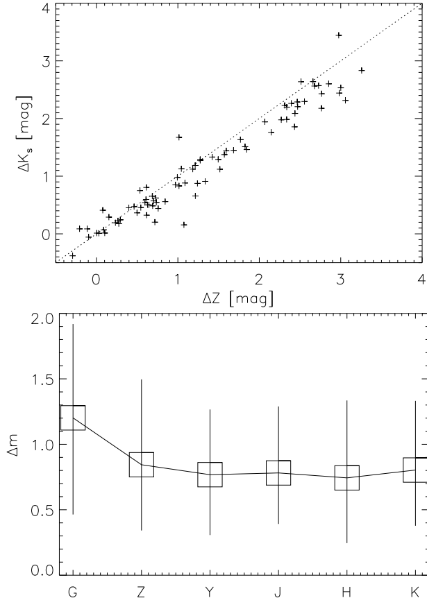
FIG. 14.— Top: comparison of magnitude differences in the Z and K_s bands for 86 physical companions with \rho > 2'' ; the dotted line marks equality. Bottom: Magnitude difference vs. wavelength for physical binaries. Squares plot the median values in each band, the bars show the first and third quartiles.
