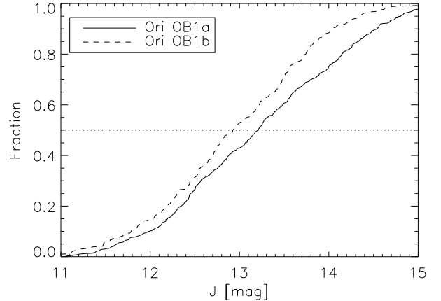
FIG. 5.— Cumulative distributions of J magnitudes for all targets classified as members (flag 1 or 2).
