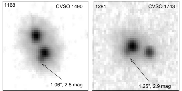
FIG. 12.— Postage-stamp H -band images of two triple systems with close faint companions, in negative rendering. Separations and \Delta J of close inner pairs are indicated. Left: target 1168 (CVSO 1490), FWHM resolution 0''.73 . Right: target 1281 (CVSO 1743), FWHM resolution 0''.87 .
