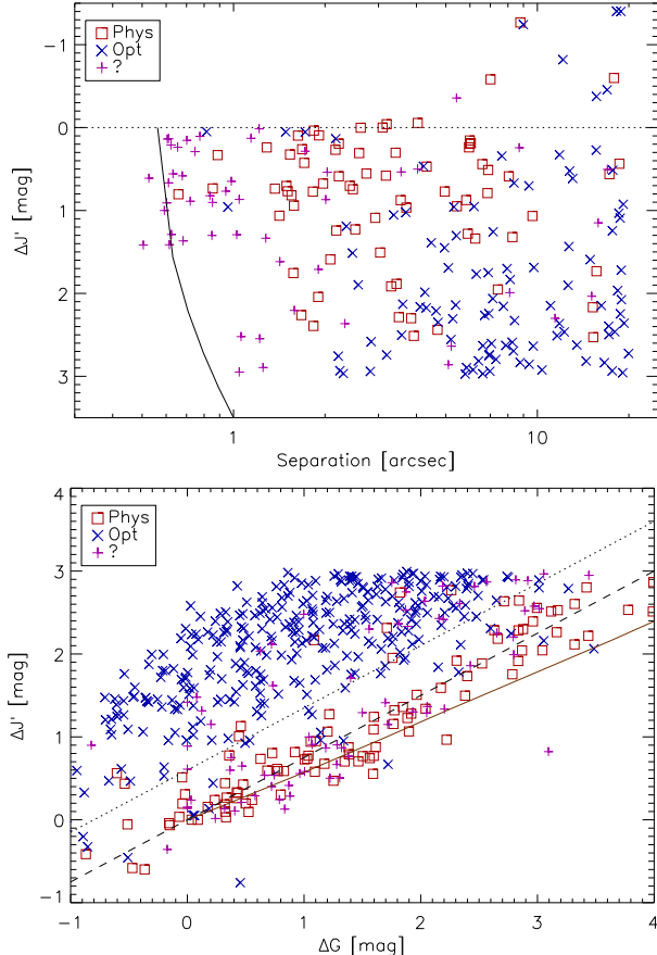
FIG. 13.— Distribution of companions in the (\rho, \Delta J') plane (top) and in the (\Delta G, \Delta J') plane (bottom). Astrometrically confirmed companions are plotted by red squares, non-members by blue crosses, and uncertain companions with p_{\text{astro}} = 0.5 by magenta plus signs. The brown solid line in the lower panel is derived from the 4 Myr PARSEC isochrone for a primary component of 0.6 M_{\odot} mass.
