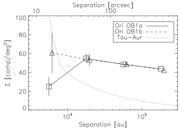
FIG. 7.— Surface density of companions vs. separation in Ori OB1a and OB1b. The dotted line shows the companion density in Taurus according to Larson (1995).
