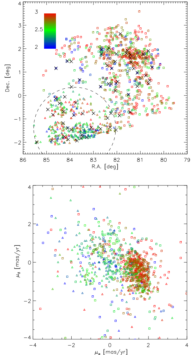
FIG. 2.— Top: location of the 1137 CVSO-VISTA objects on the sky (squares for OB1a, triangles for OB1b). The points are colored by parallax in the range from 2 to 3 mas, as shown by the color bar. Black crosses are stars without GDR2 parallaxes. The dashed circle indicates the approximate boundary of the Ori OB1b group. Bottom: distribution of the sample of 1078 objects with GDR2 astrometry in proper motion space. The symbols and colors are the same as in the top panel.
