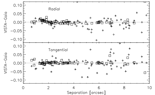
FIG. 10.— Comparison of double-star astrometry between VISTA Orion and Gaia. Squares are astrometrically confirmed association members, pluses are other (mostly optical) companions with \Delta G < 3 mag. The top plot compares separations, the lower plot shows the tangential difference \rho \sin \Delta\theta . The axis scale is in arcseconds.
