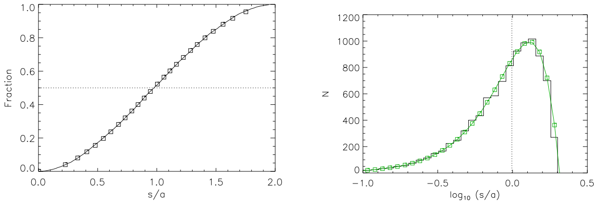
FIG. A1.— Left: cumulative distribution of the ratio s/a (line) and its analytic model (squares) for thermal eccentricity distribution. Right: histogram of the same data and their model (green squares and line); vertical dotted line marks the median.
