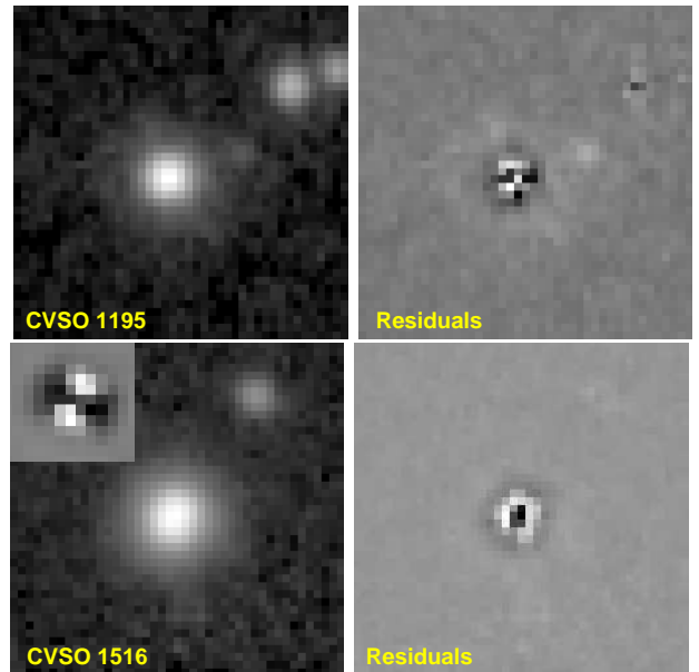
FIG. 8.— Modeling the postage-stamp images by Moffat functions. The images are shown on the left, the residuals on the right. Top: the image of target 1027 (CVSO 1195) in the H band with three stars. Note another faint star in-between that has been ignored. Bottom: the image of target 1176 (CVSO 1516) in the J band, with an insert showing residuals for the main star indicating the elongation. The residuals after fitting three stars (on the right) are smaller.
