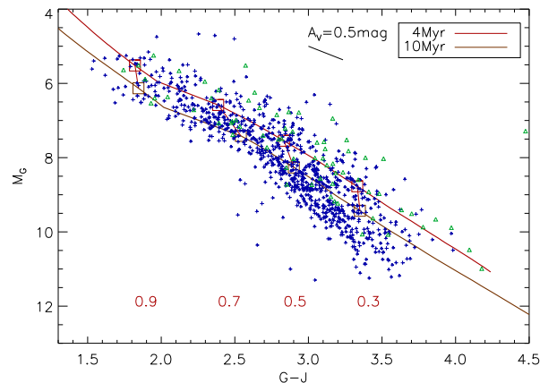
FIG. 6.— Color-magnitude diagram. Known binaries with separations less than 5'' are plotted by green triangles, other stars by blue crosses. Absolute magnitudes have been derived for each star based on its parallax. Two PARSEC isochrones for solar metallicity are plotted. The squares on the isochrones and numbers mark masses from 0.3 to 0.9 M_\odot . The line marks the effect of an A_V = 0.5 mag extinction.
