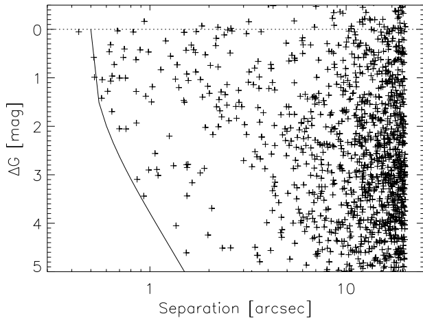
FIG. 9.— Separation versus \Delta G of companions found in Gaia within 20'' . The line shows the detection limit \Delta G < 5(\rho - 0.5)^{0.4} that approximates the detection limit at 50% probability found by Brandeker & Cataldi (2019).
