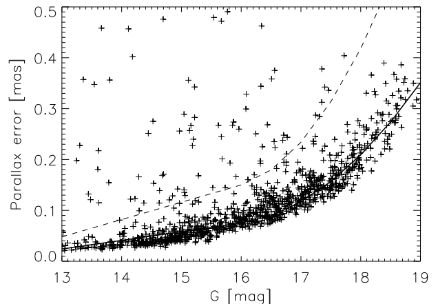
FIG. 3.— Parallax errors vs. G magnitude (crosses). The full line is \sigma_0(G) defined by equation. 1, the dashed line represents 2\sigma_0(G) .
