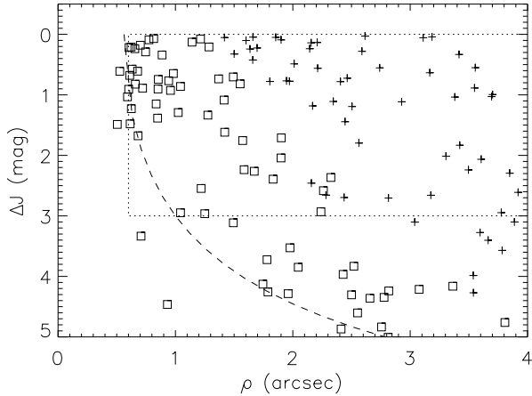
FIG. 11.— Location of companions in the (\rho, \Delta J) plane. Squares denote pairs found in our image analysis, crosses plot companions found both in the images and in the VISTA Orion catalog. The dashed line is the empirical detection limit (eq. 4), the dotted rectangle marks the limits of our statistical analysis.
