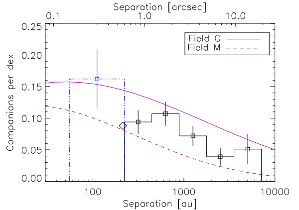
FIG. 19.— Distribution of separation in the full sample. The dash-dot line shows the result for the SOAR sample. The diamond is the companion frequency in the ONC from Reipurth et al. (2007). A distance of 370 pc is used.
