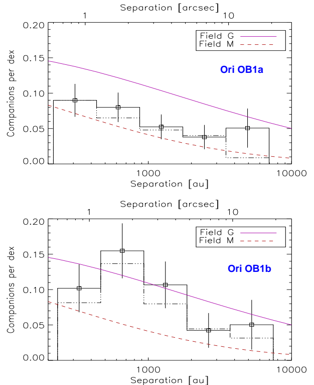
FIG. 18.— Companion frequency vs. separation (fraction per decade) in Ori OB1a (top) and Ori OB1b (bottom). The full line corresponds to binaries with \Delta J < 3 mag, the dash-dot line to binaries with \Delta J < 2 mag. The log-normal distributions for field stars (solid and dashed curves) are described in the text.
