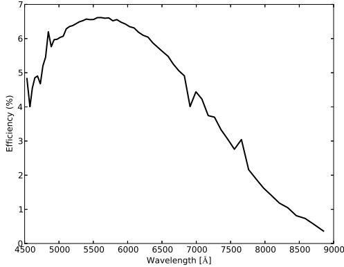
Fig. 7.— Spectral efficiency of CHIRON in fiber mode measured on August 1, 2013 (median for three standard stars, with three exposures of each star). The atmospheric extinction was removed, so that the curve includes only telescope, spectrograph, and detector.
