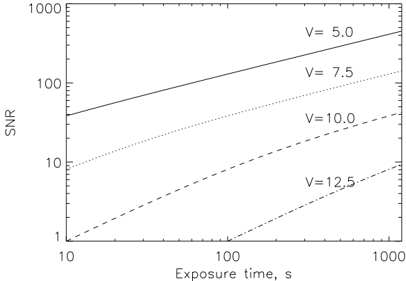
Fig. 8.— Signal-to-noise ratio per pixel vs. stellar V-band magnitude and exposure time in the slicer mode (at 550 nm near the blaze peak).
