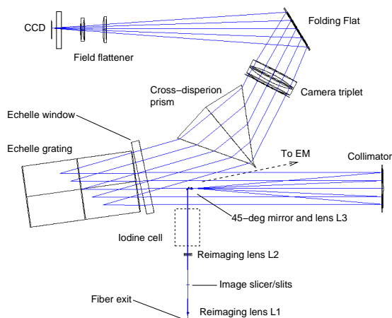
Fig. 1.— Layout of the CHIRON optics (see text).
