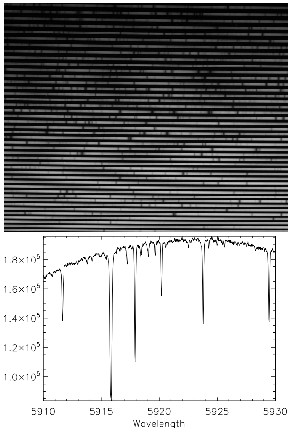
Fig. 5.— Top: Fragment of the spectrum of a nearby G8V star HD 20794 (82 Eri, V = 4.26 ) in slicer mode recorded on October 8 2011 with a 10-minute exposure. Bottom: portion of the extracted order with signal-to-noise ratio (SNR) of \sim 400 .
