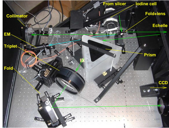
Fig. 2.— Optical elements of CHIRON and the light path.
