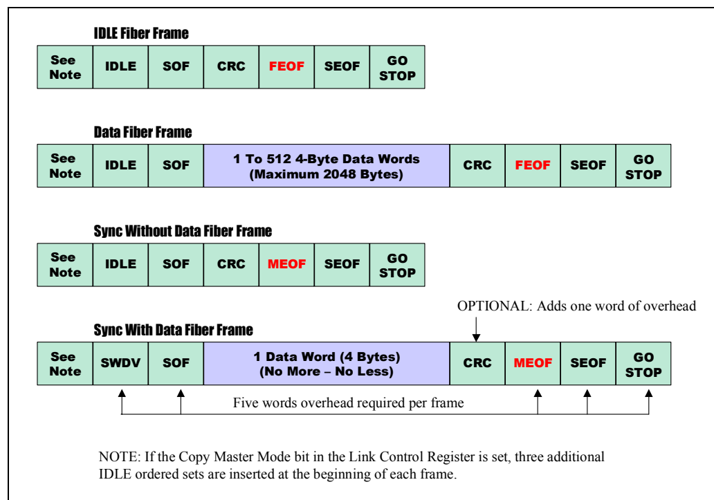
Figure D-1 VITA 17.1 Framing Protocol
