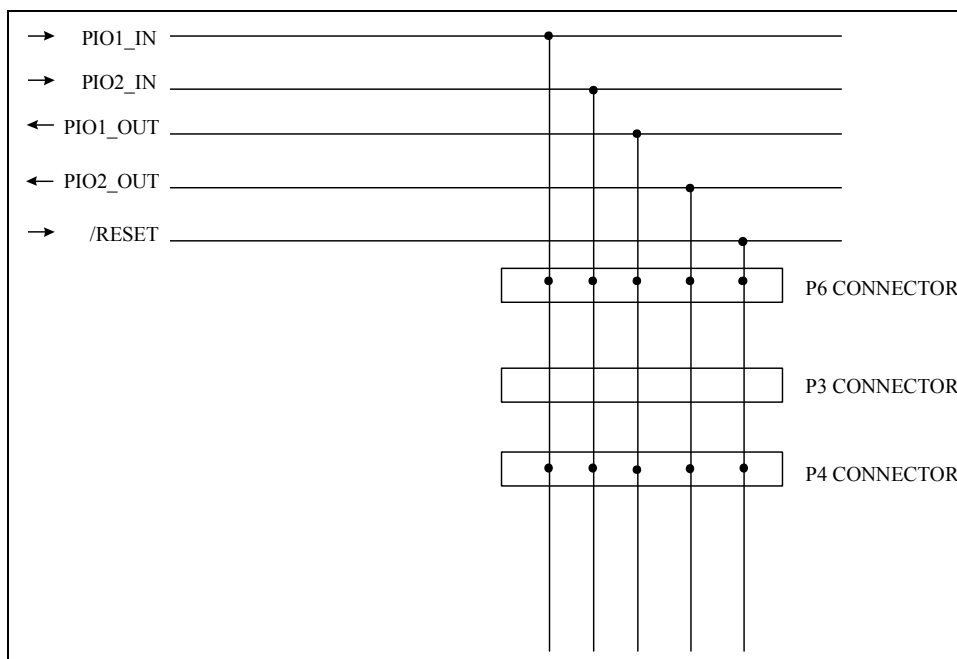
Figure G-5 PIO Line Interconnectivity
