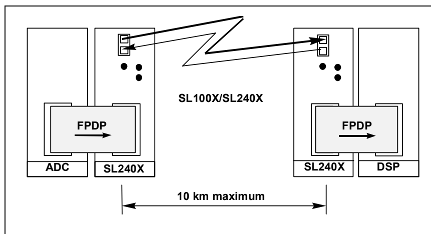
Figure 2-7 FibreXtreme SL240X Extending FPDP
