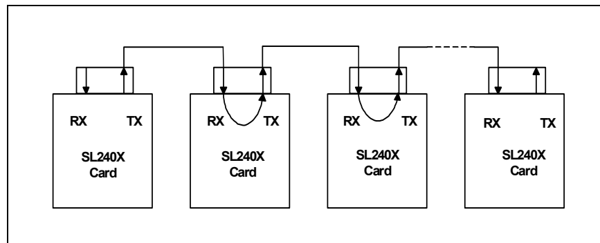
Figure 2-9 Chained Topology
