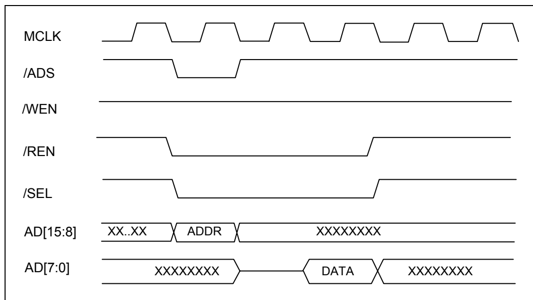
Figure G-7 Microcontroller Single Read
