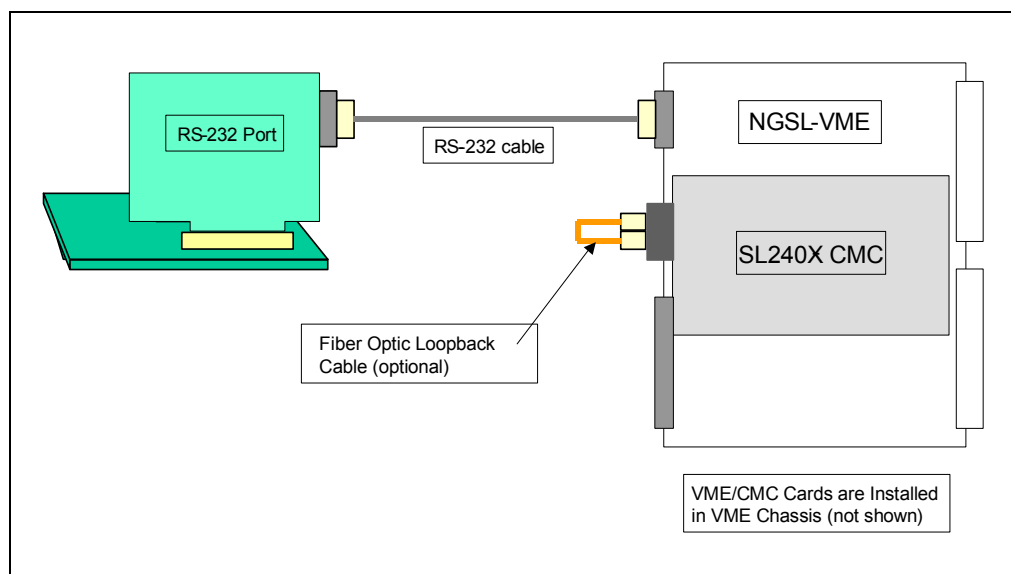
Figure C-1 NGSL VME card Configuration Environment
