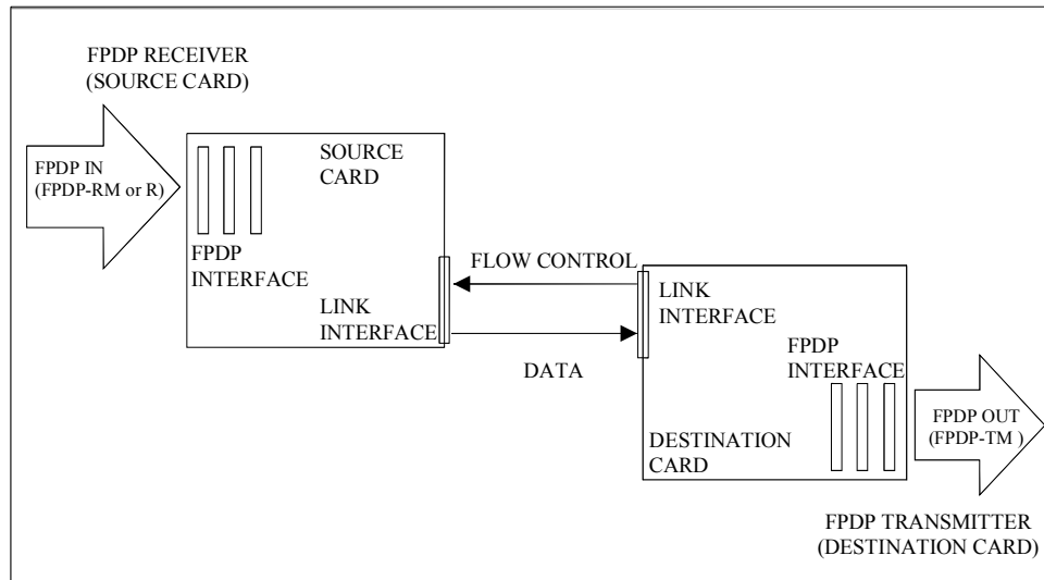
Figure G-2 FPDP and SL240X Terminology
