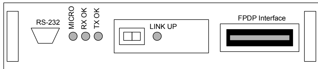
Figure 2-12 Status LEDs on SL240X VME and Rehostable CMC Cards
