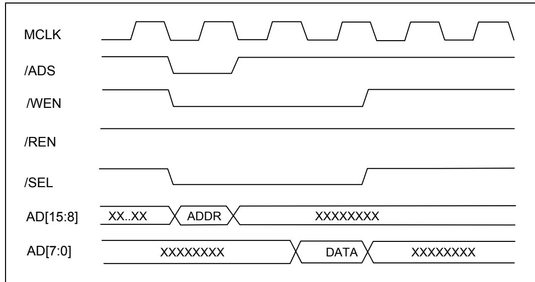
Figure G-8 Microcontroller Single Write
